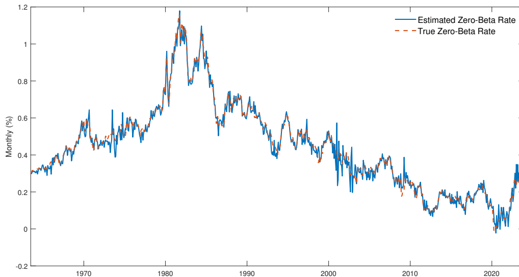
Figure. 6. Estimated Zero-Beta Rate vs True Zero-Beta Rate (Fama-MacBeth)
