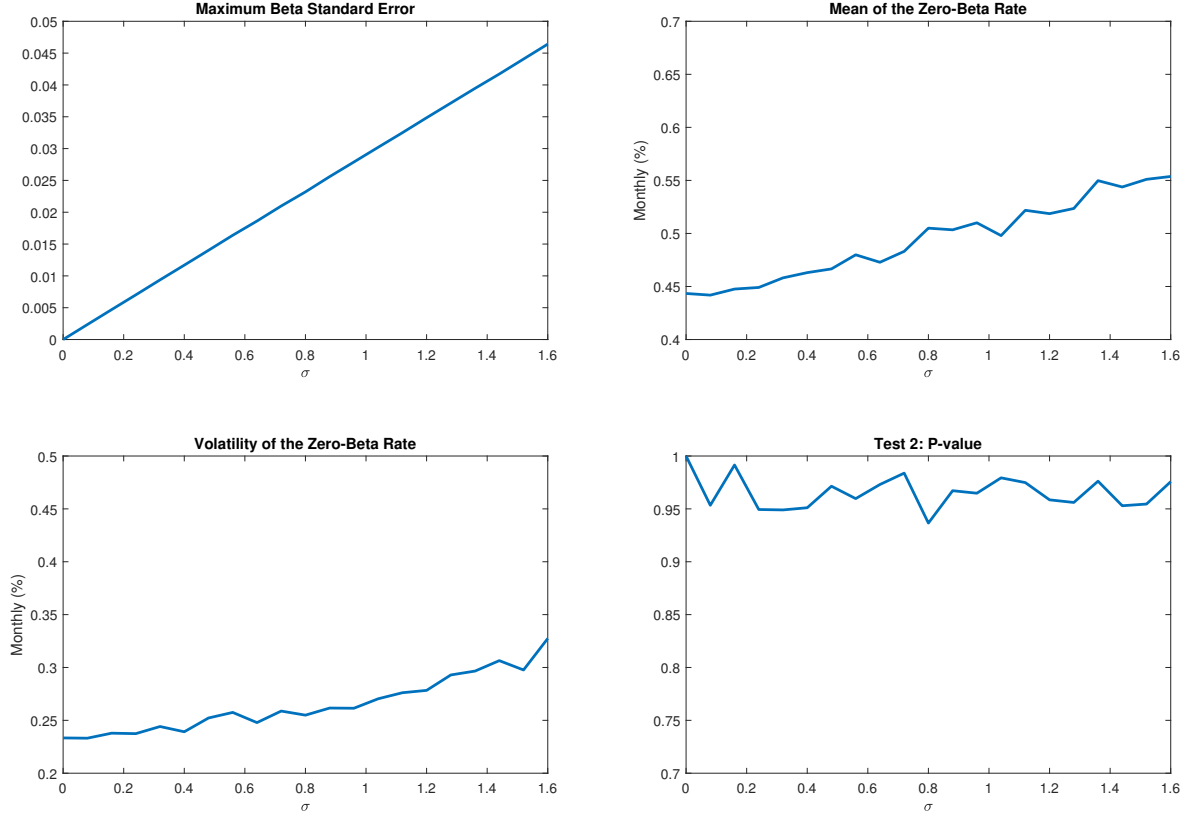
Figure. 9. Estimated Zero-Beta Rate (DHKW), Errors-in-Variables
