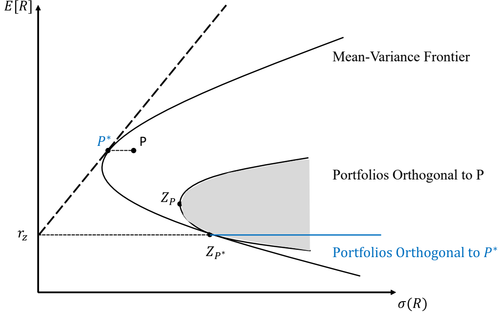
Figure. 3. The Mean-Variance Frontier and Zero-Beta Frontiers
